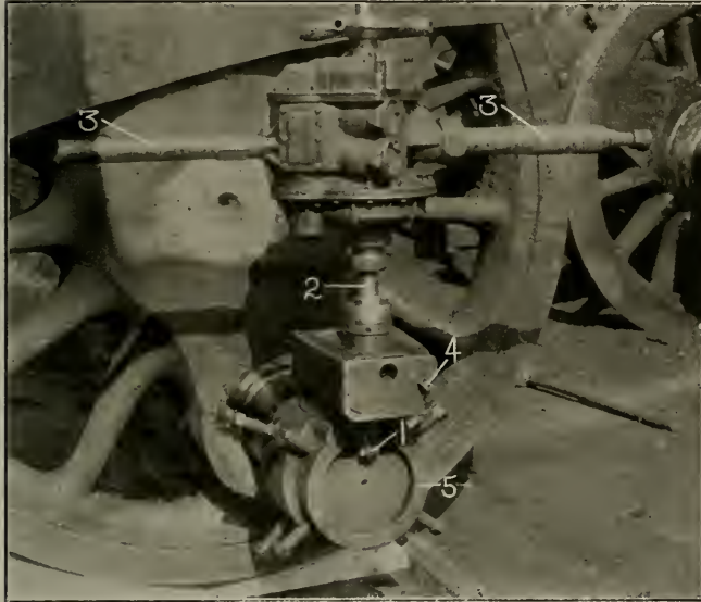
PORTABLE CRANKPIN MILLER
